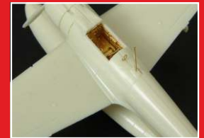
BRL144045 A6M2-N Rufe PE set for SWEET kit ( 2sets)
