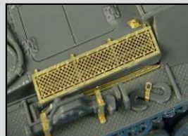
HLX48004 Stug.III.ausf.B-grills photoetched parts for TAMIYA kit
