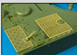
HLX48031 TIGER I LATE grills-AFV photoetched parts for AFV
