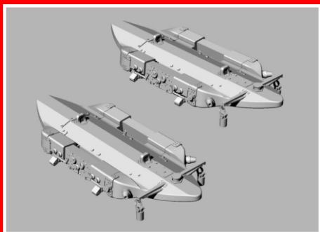
BRL48168 BRU-57 canted Vertical Ejector Rack -resin set for US planes (2 pcs)
