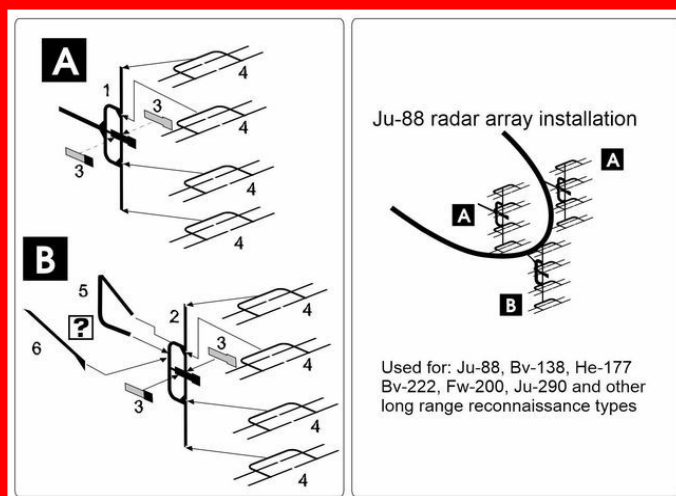
BRL144212 FUG-220 Lichtenstein PE set of german aircraft radar antennas
